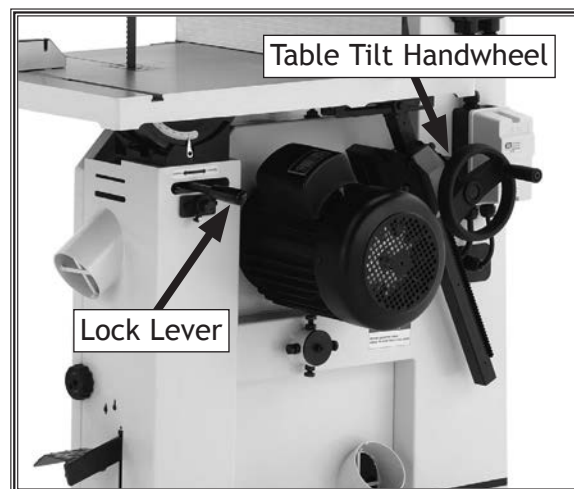
Figure 54. Table tilt controls.
