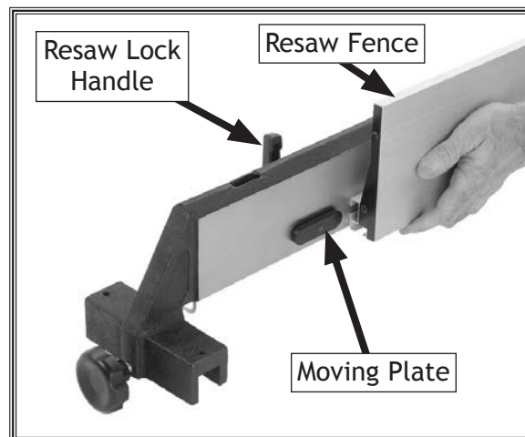
Figure 43. Attaching resaw fence to standard fence.
