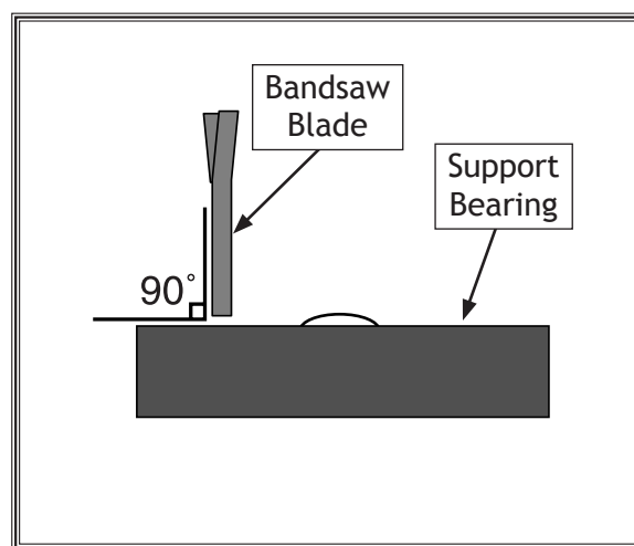
Figure 32. Illustration of blade set perpendicular (90°) to the support bearing face.
