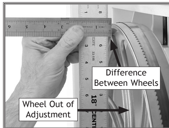
Figure 76. Determining distance needed to shim upper wheel.
