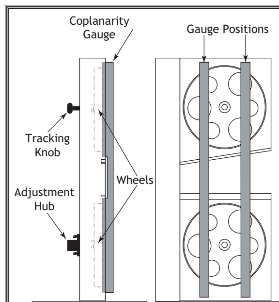
Figure 74. Checking for coplanarity.
