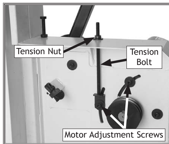
Figure 68. Motor mount bolts and tension bolt. (Lower wheel removed for clarity.)
