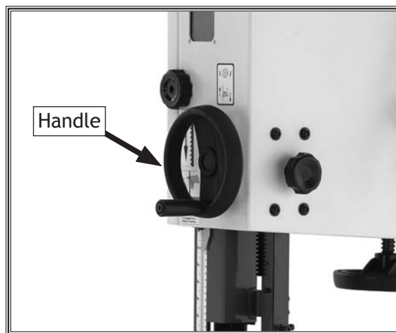
Figure 16. Guide post handwheel installed.
