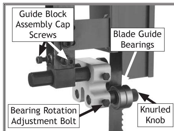
Figure 27. Upper blade guide controls (rear view).
