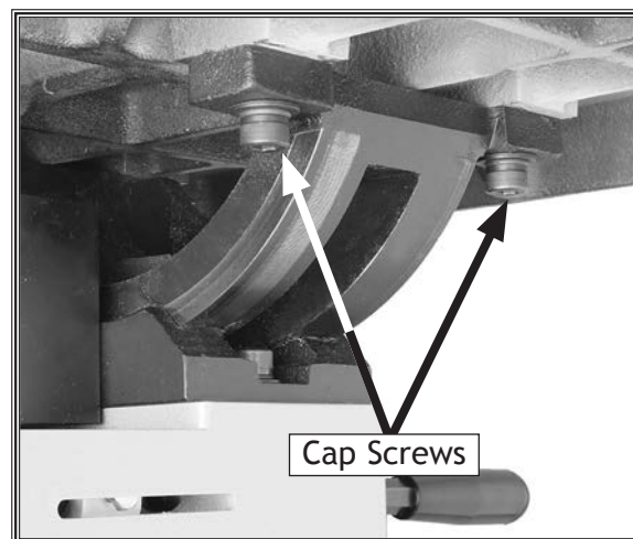
Figure 36. Cap screws securing table to trunnion.
