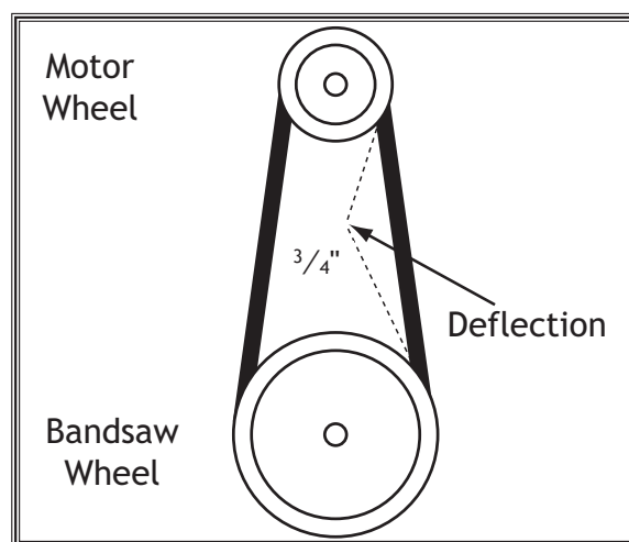
Figure 67. V-belt deflection.
