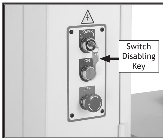
Figure 23. W1770 switch disabling key and ON/OFF switch
