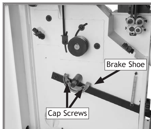
Figure 72. Brake shoe location.
