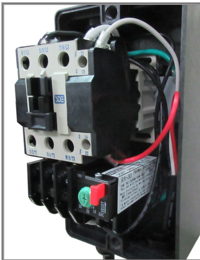
Figure 80. Magnetic switch.
