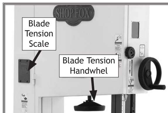
Figure 26. Front blade tensioning controls.
