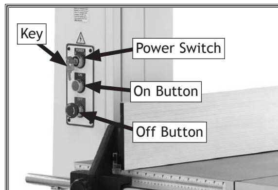
Figure 45. W1770 control panel features.
