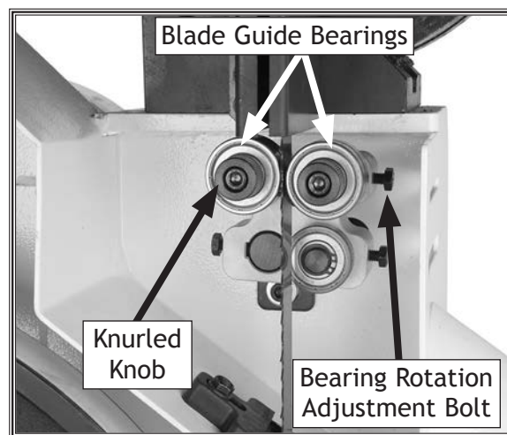
Figure 30. Lower blade guide controls (front view).
