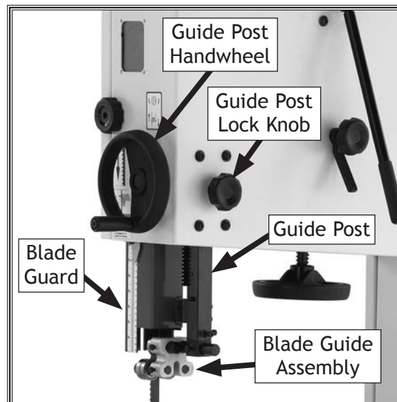
Figure 51. Guide post controls.
