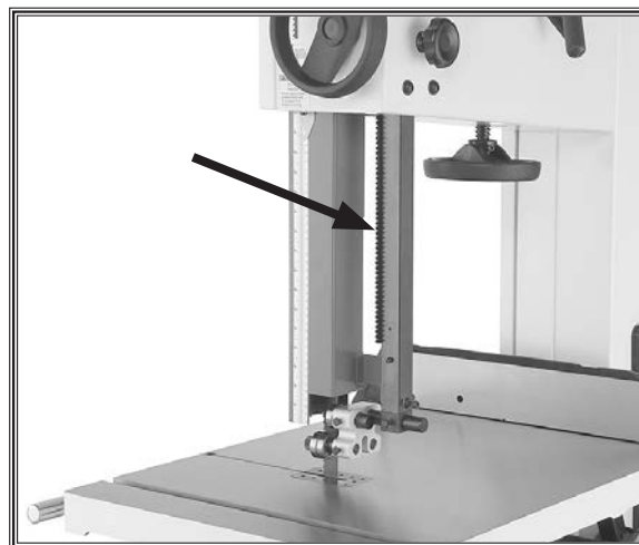
Figure 63. Rack lubrication location.
