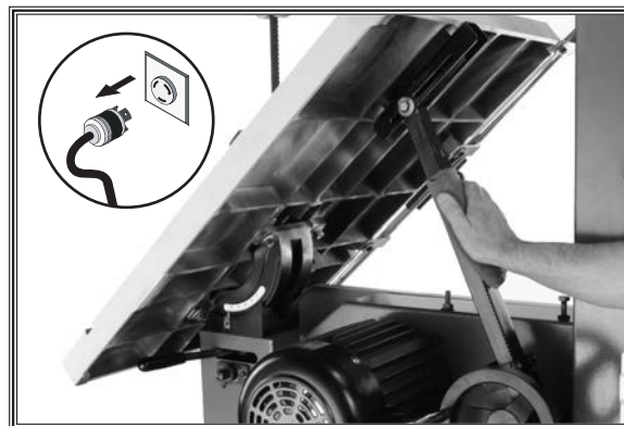
Figure 65. Table tilt rack and pinion assembly.
