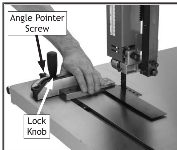
Figure 42. Example of squaring miter gauge to blade.
