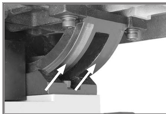
Figure 66. Trunnion lubrication location.
