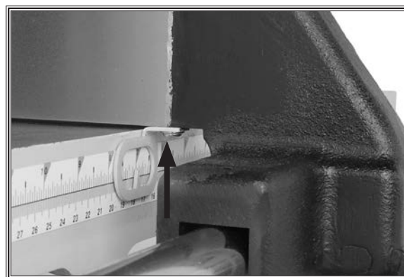
Figure 41. Fence pointer adjustment screw.
