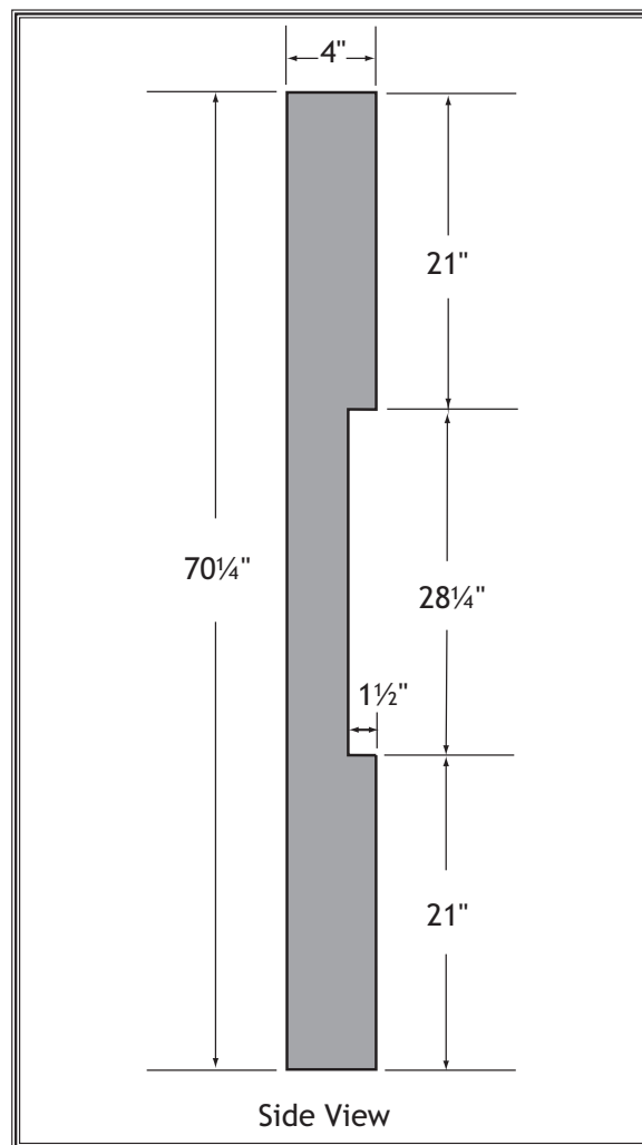
Figure 73. Dimensions of coplanarity gauge.
