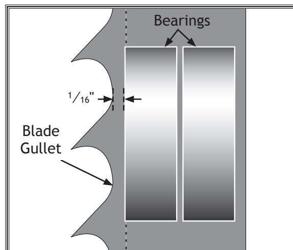
Figure 29. Lateral adjustment of blade guides.
