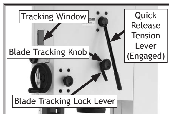
Figure 18. Rear blade tensioning and tracking controls.
