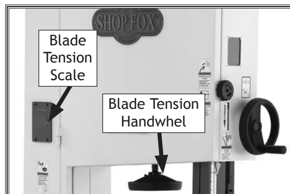
Figure 17. Front blade tensioning controls.
