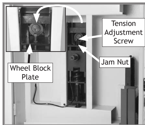
Figure 70. Quick release tension lever adjustment screw.
