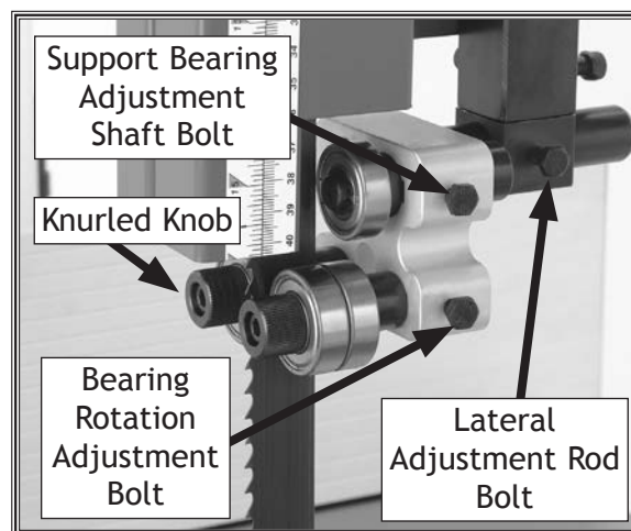
Figure 28. Upper blade guide controls (front view).
