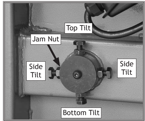
Figure 77. Lower wheel adjustment hub.
