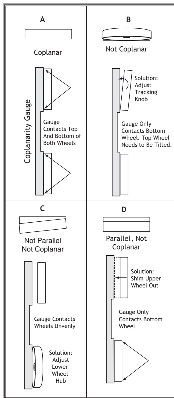
Figure 75. Coplanar diagram.
